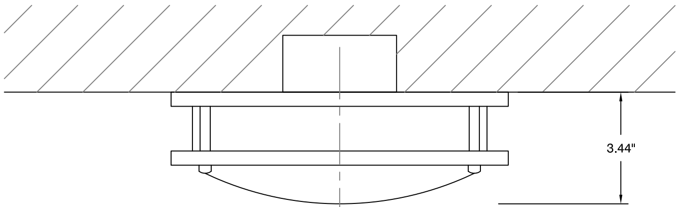
FRONT VIEW
