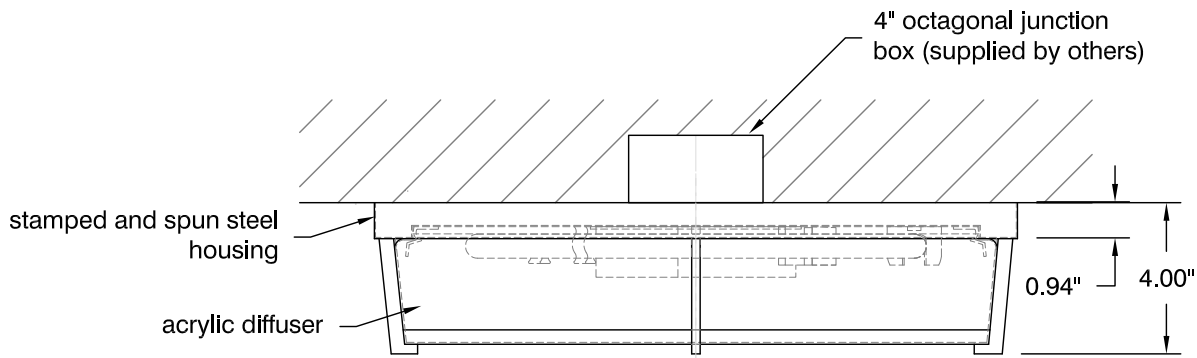
SIDE VIEW
