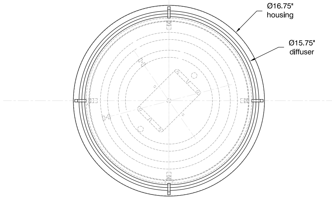
BOTTOM VIEW
