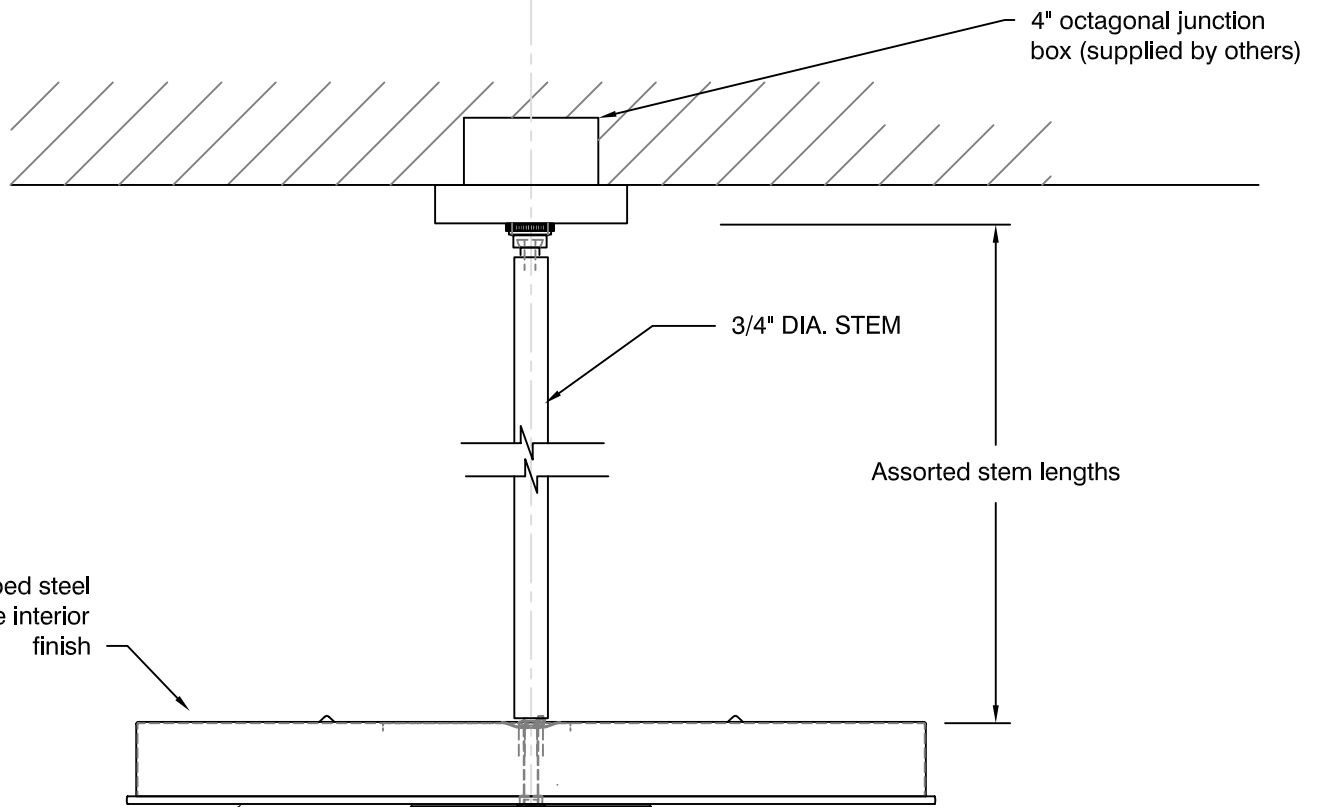
SIDE VIEW
