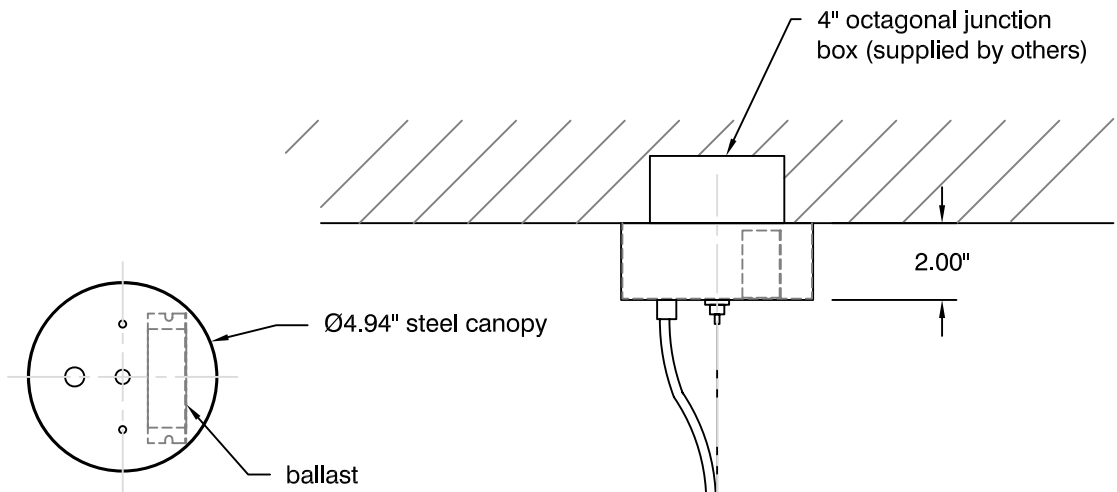
TOP VIEW (canopy)
