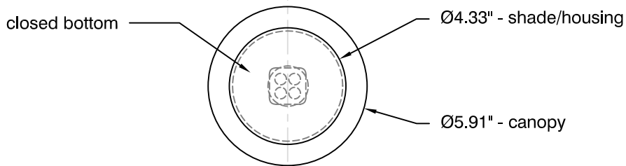
BOTTOM VIEW
