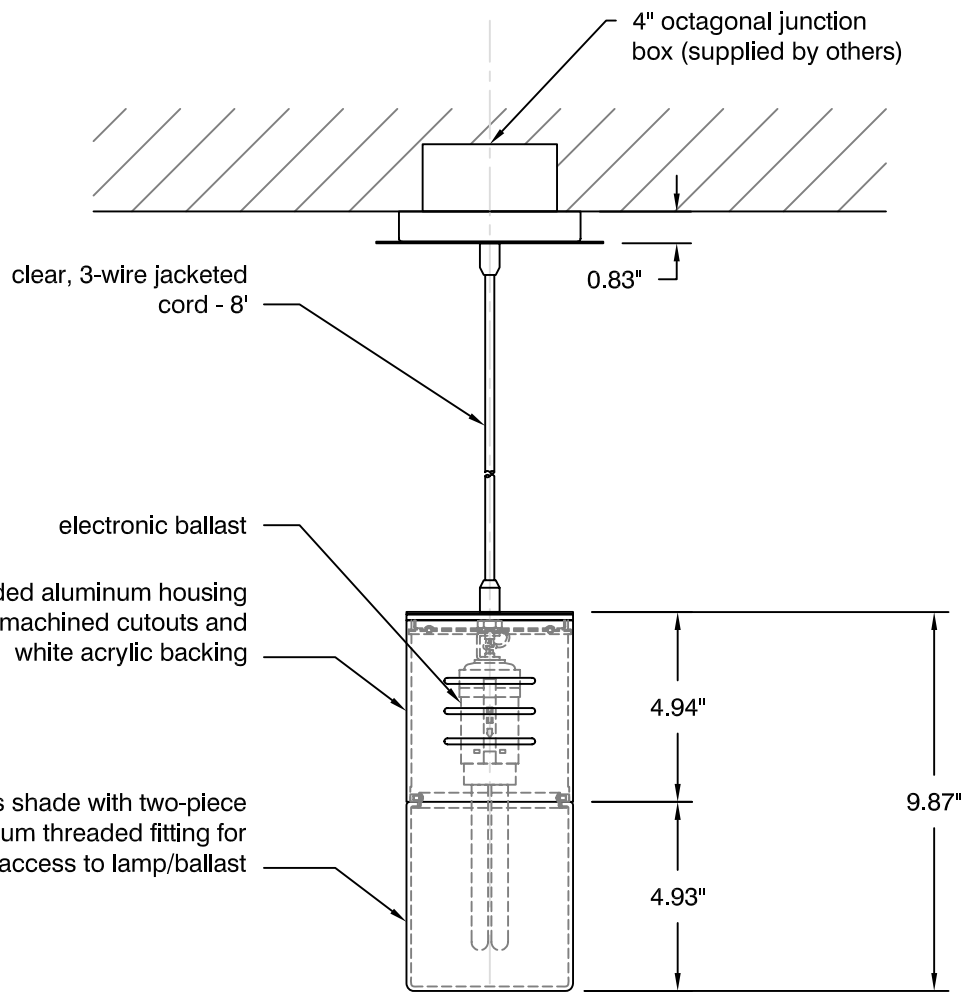
SIDE VIEW
