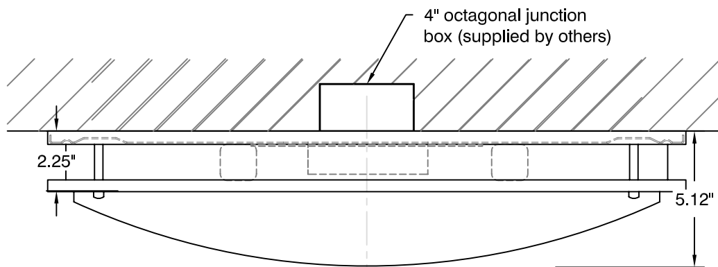
SIDE VIEW
