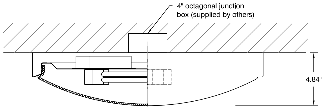
SIDE VIEW
