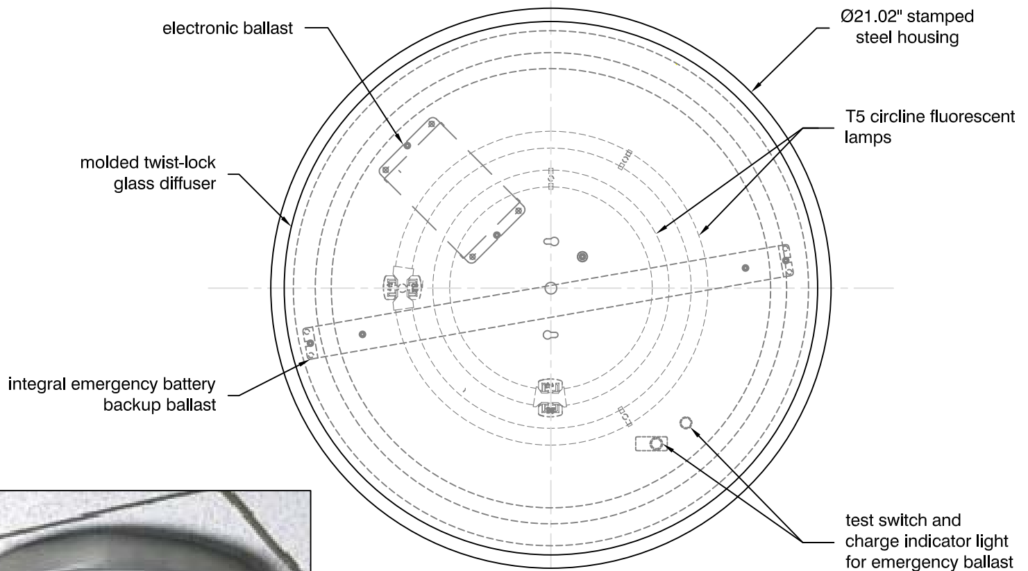
BOTTOM VIEW
