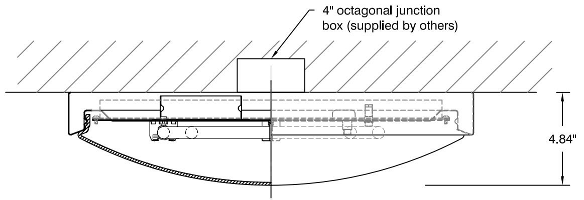
SIDE VIEW
