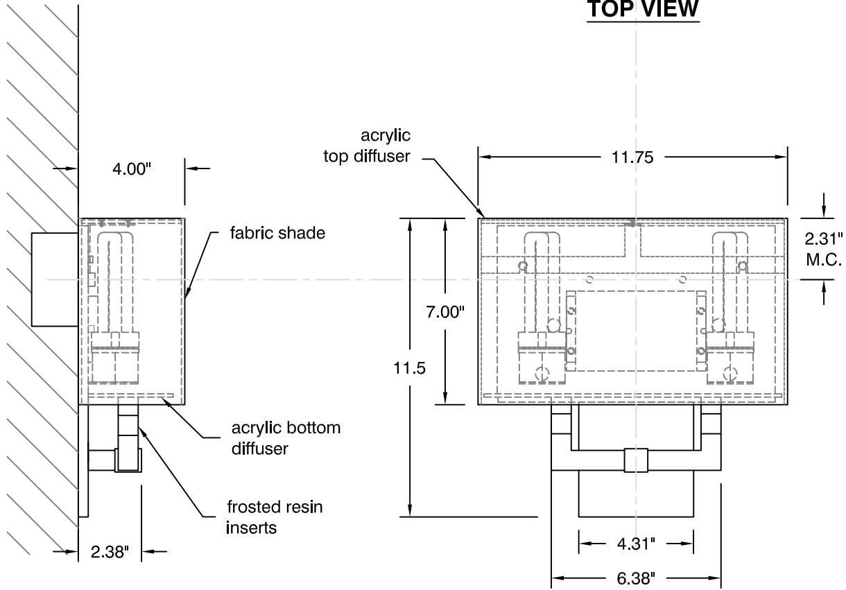
SIDE VIEW
