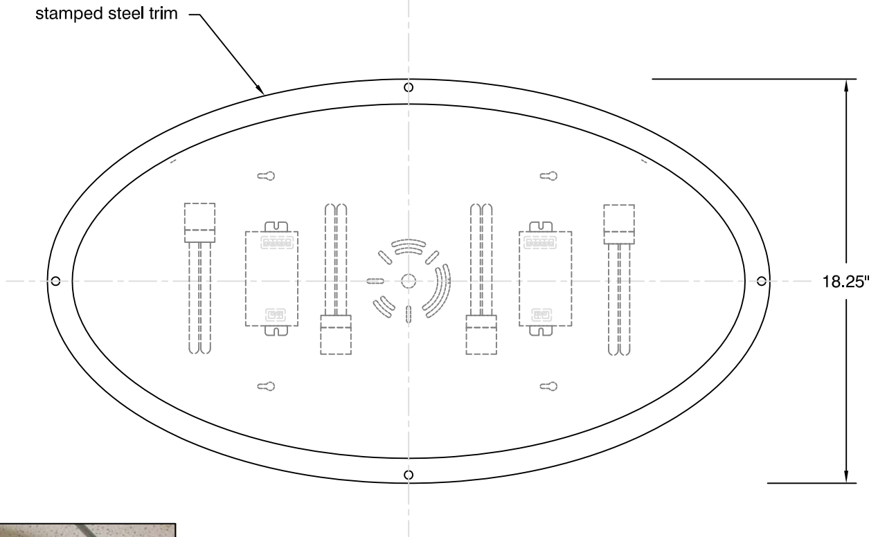
BOTTOM VIEW
