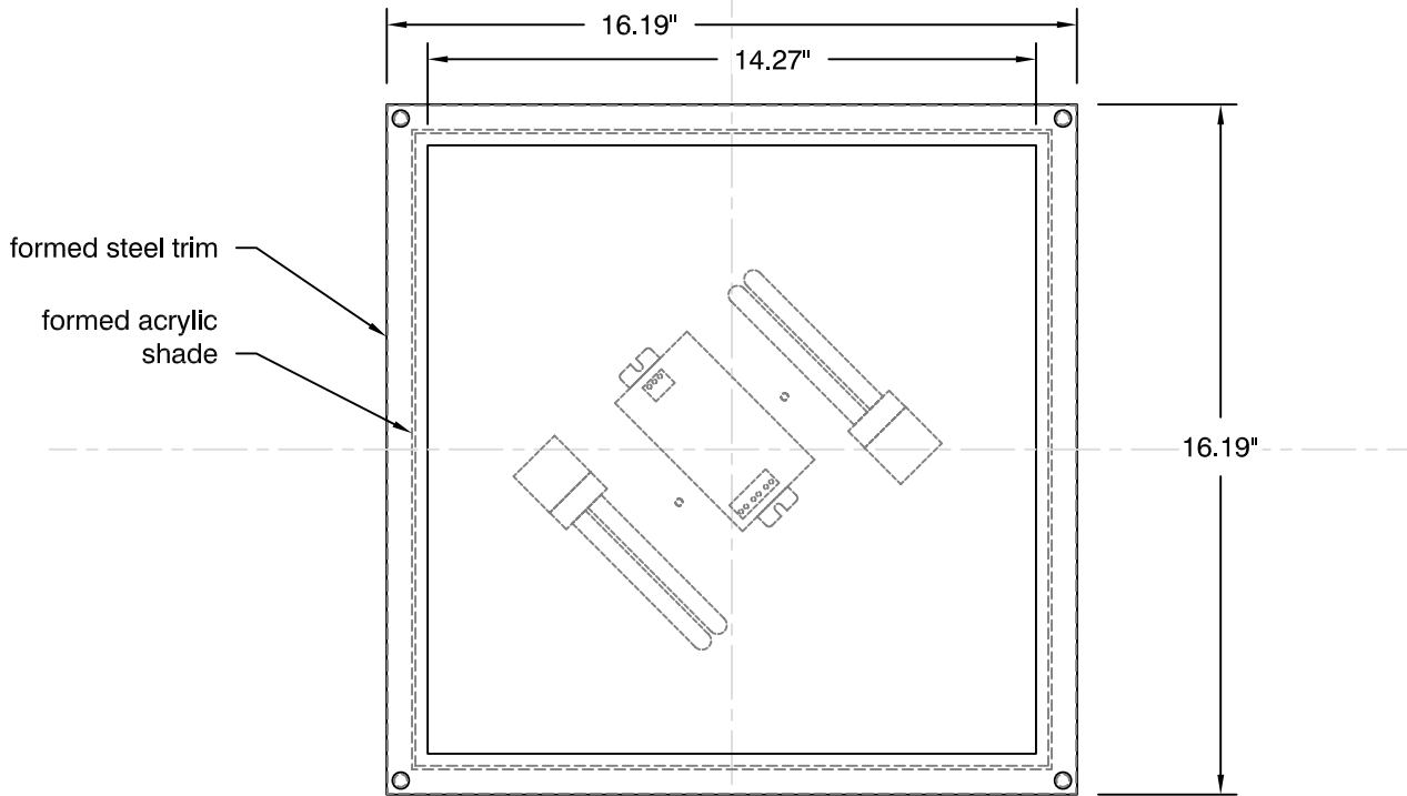
BOTTOM VIEW
