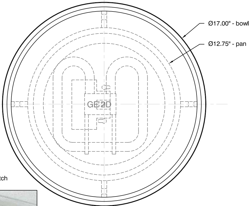
BOTTOM VIEW
