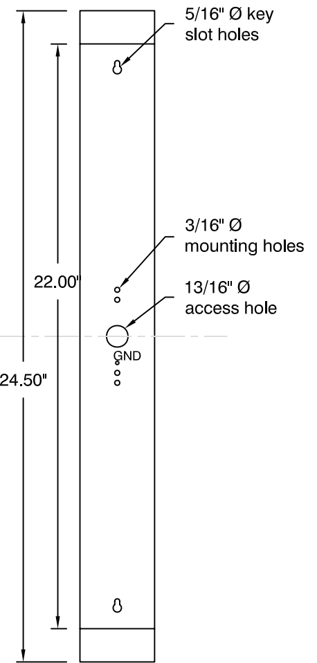
MOUNTING PLATE
