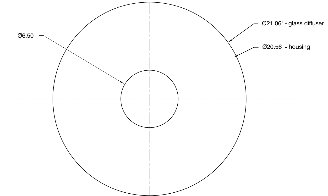
BOTTOM VIEW
