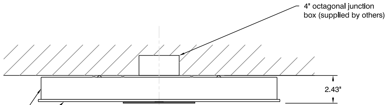
SIDE VIEW
